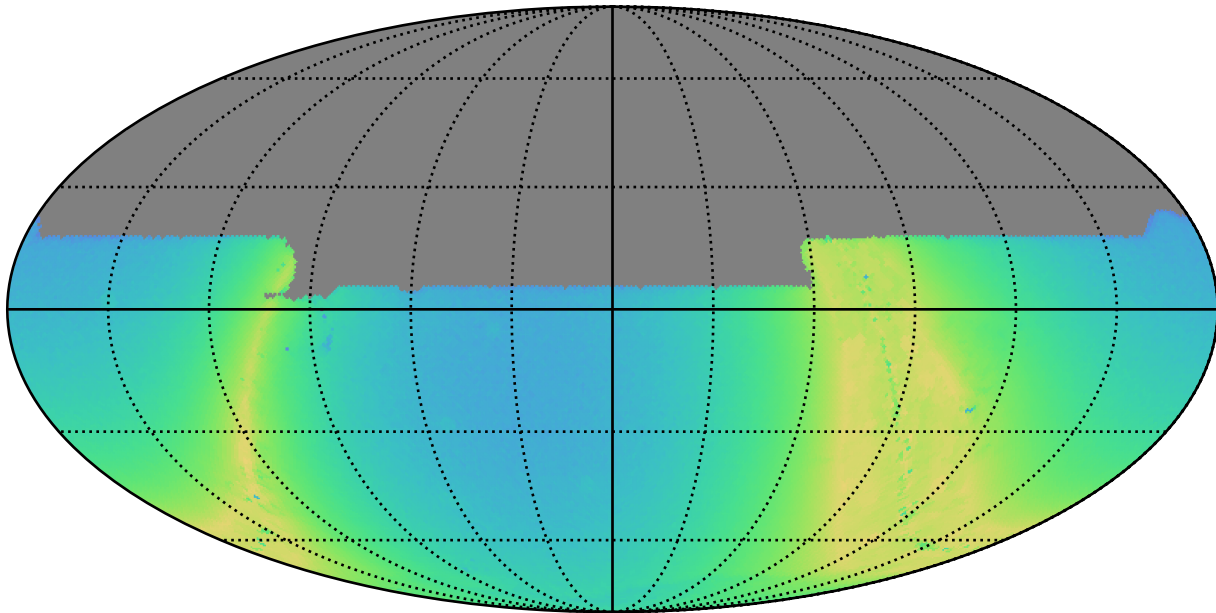
no_high_blob_v3.3_10yrs y: N stars to Precision 0.20
