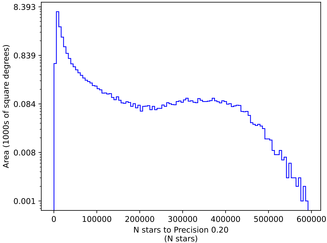
no_high_blob_v3.3_10yrs y: N stars to Precision 0.20
