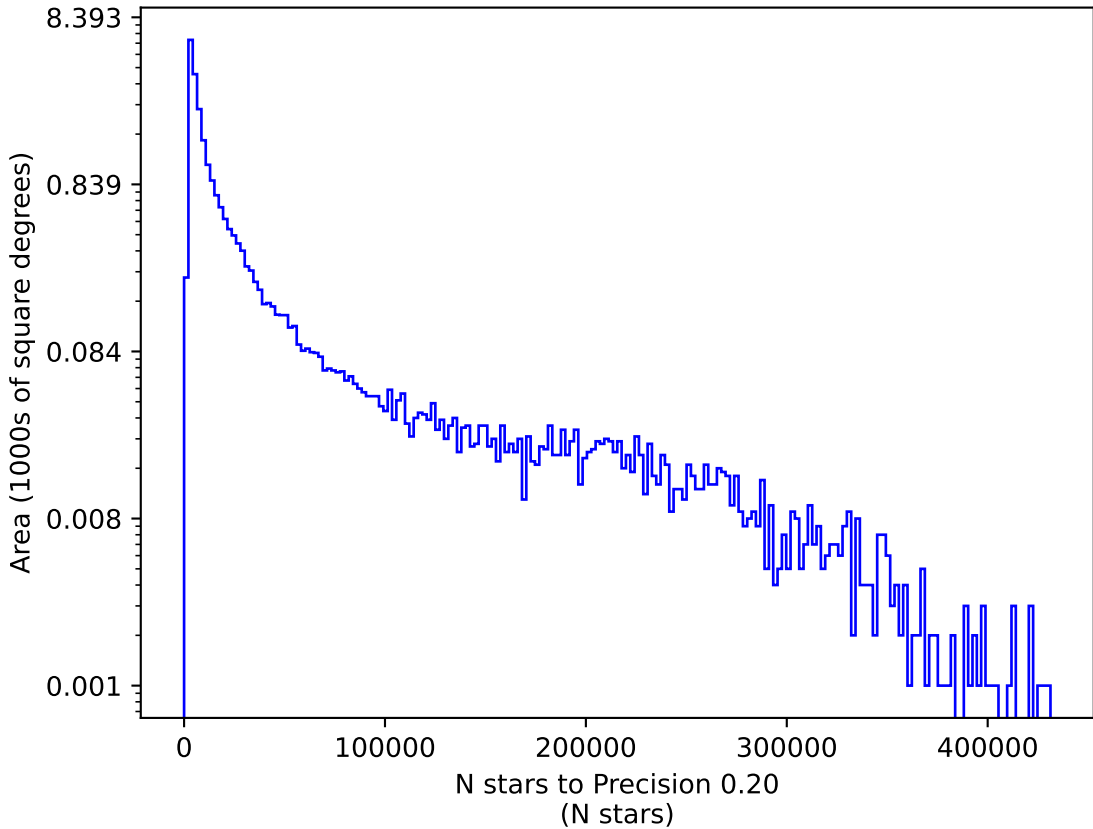
no_high_blob_v3.3_10yrs u: N stars to Precision 0.20
