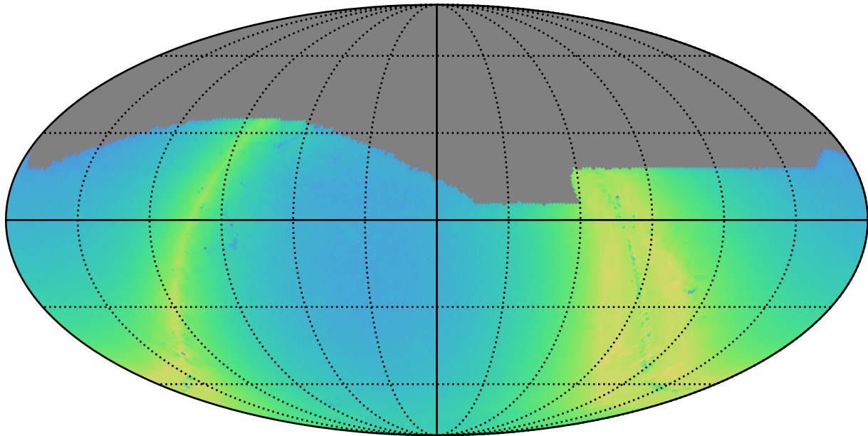
no_high_blob_v3.3_10yrs r: N stars to Precision 0.20
