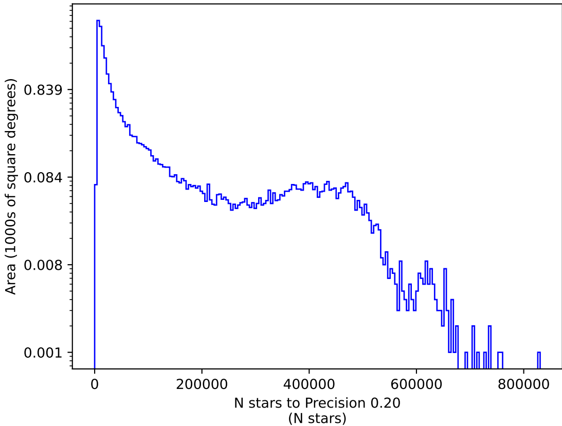
no_high_blob_v3.3_10yrs r: N stars to Precision 0.20
