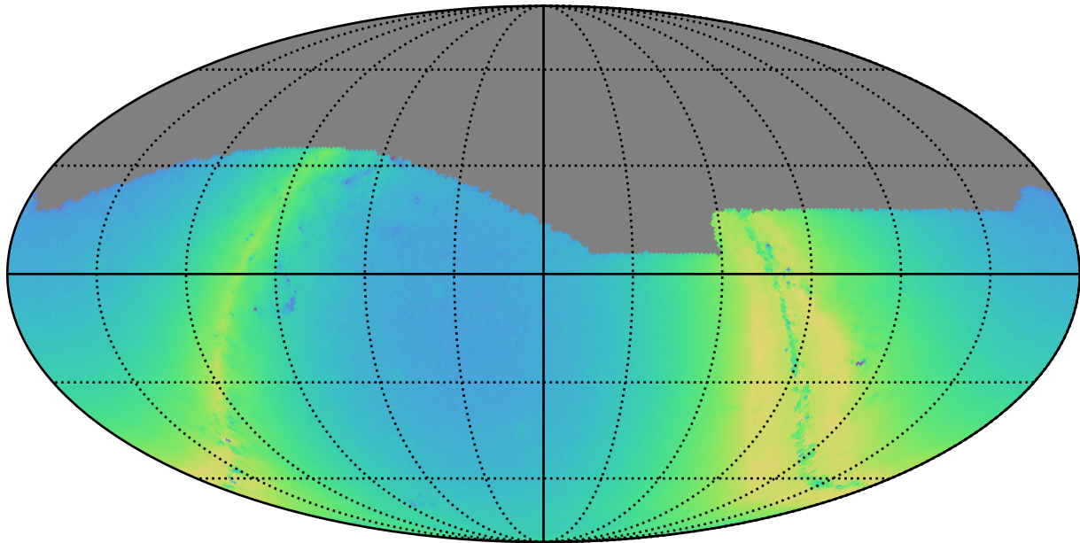
no_high_blob_v3.3_10yrs g: N stars to Precision 0.20
