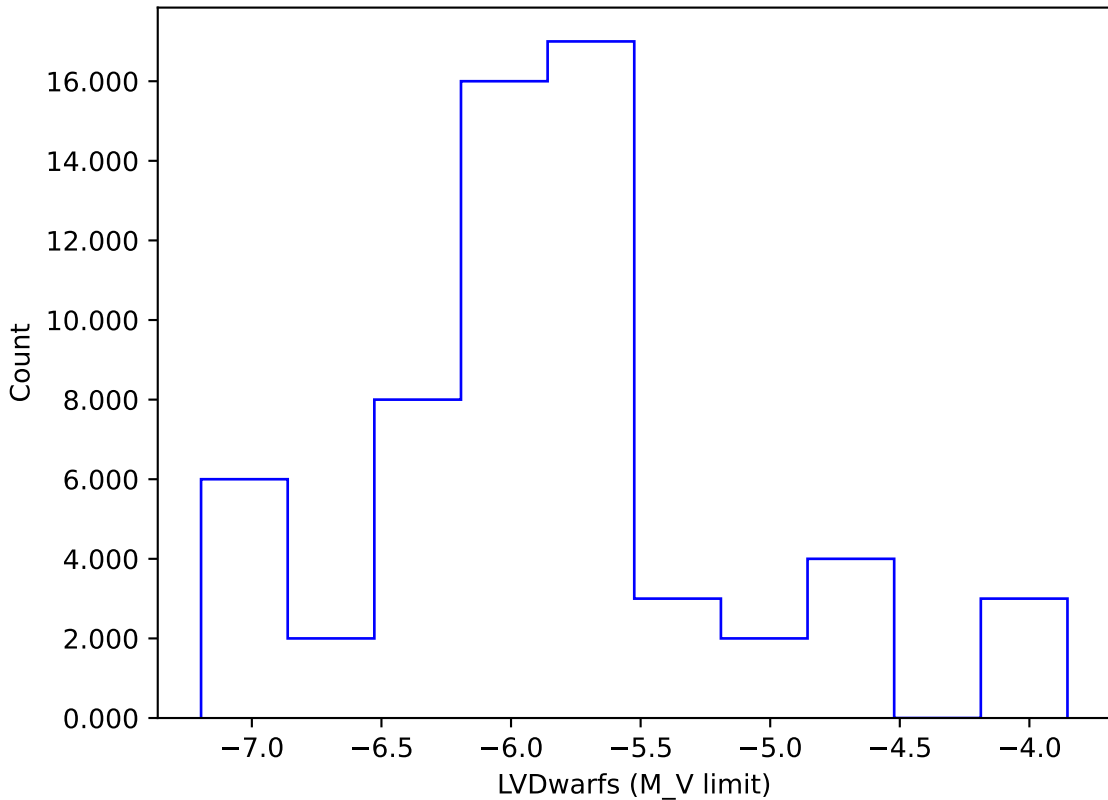
no_high_blob_v3.3_10yrs gi: LVDwarfs
