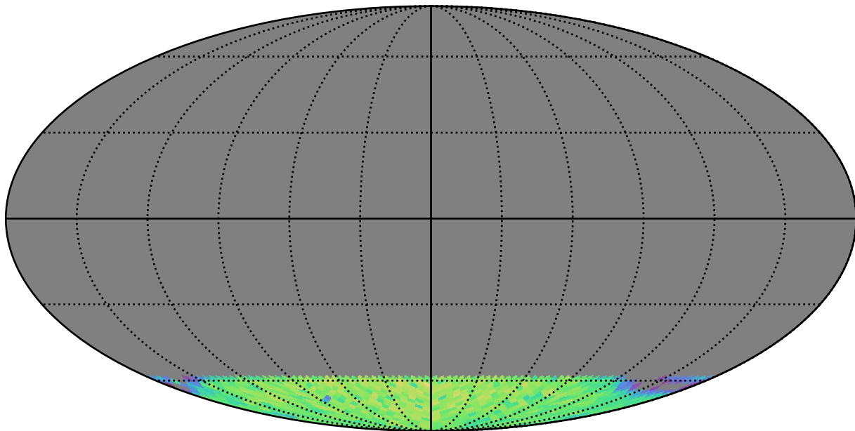
no_high_blob_v3.3_10yrs gi SCP: LVDwarfs
