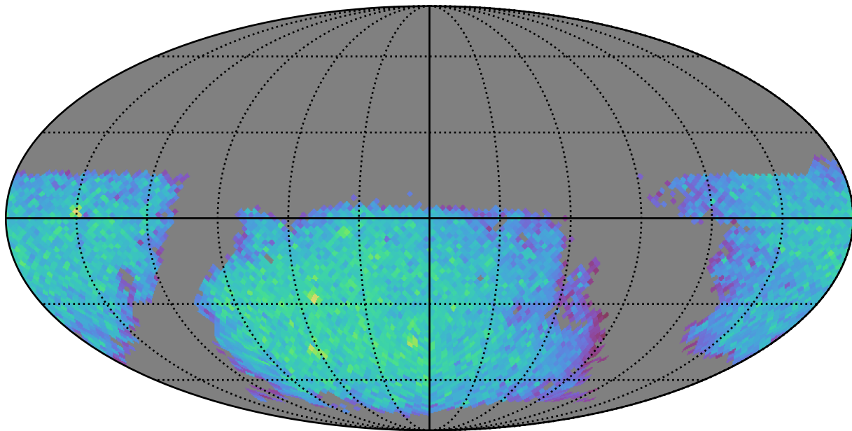
no_high_blob_v3.3_10yrs gi: LVDwarfs
