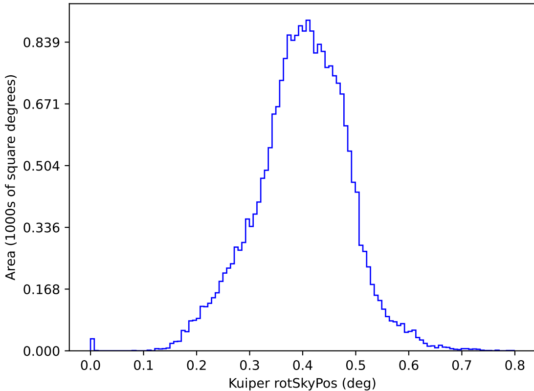
no_high_blob_v3.3_10yrs y: Kuiper rotSkyPos
