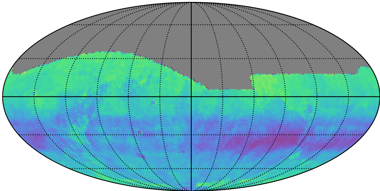
no_high_blob_v3.3_10yrs r: Kuiper rotSkyPos
