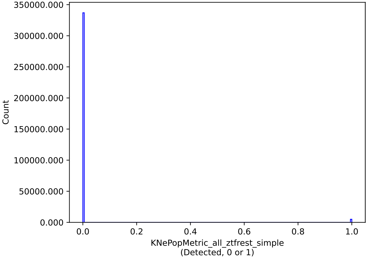
no_high_blob_v3.3_10yrs all models: KNePopMetric_all_ztfrest_simple
