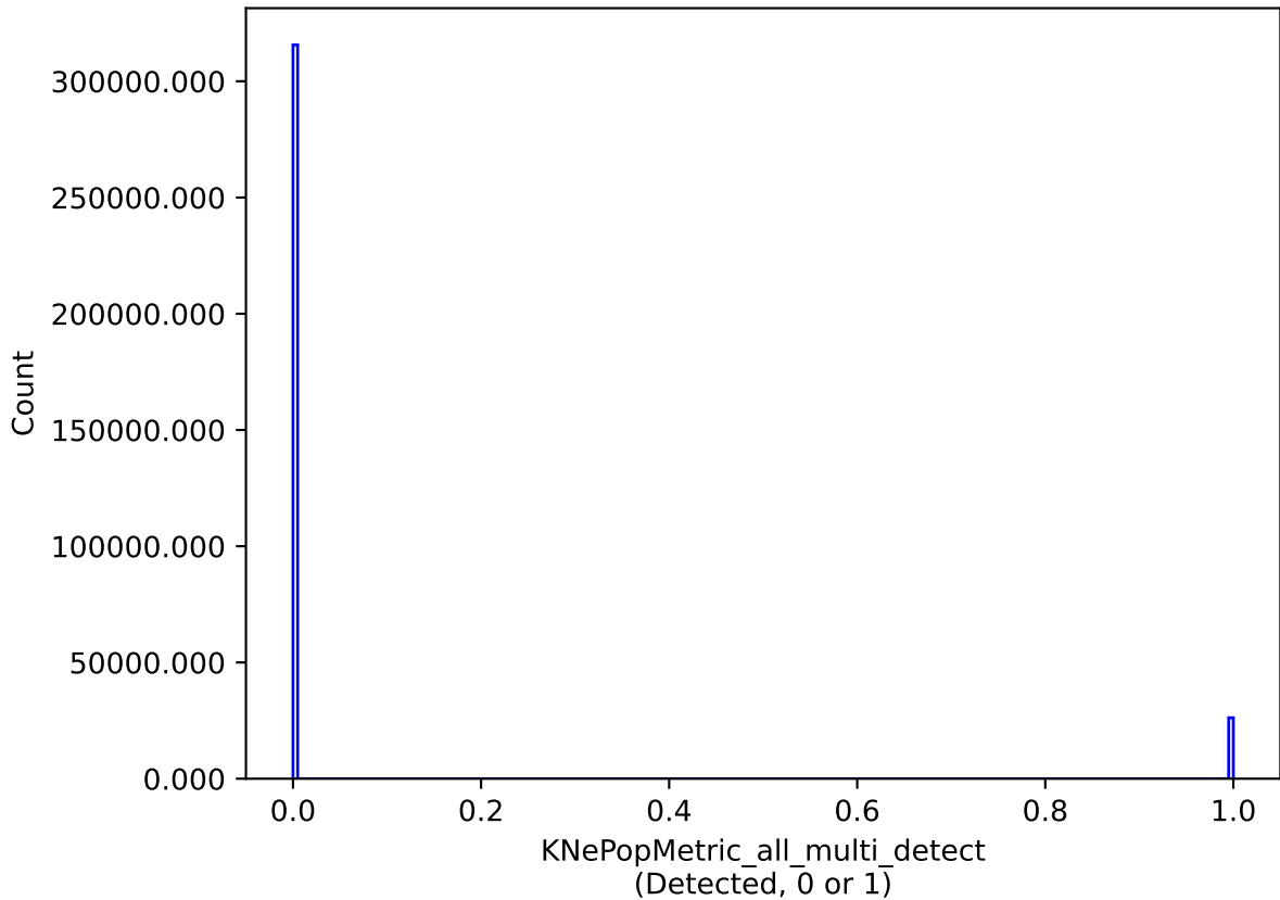
no_high_blob_v3.3_10yrs all models: KNePopMetric_all_multi_detect
