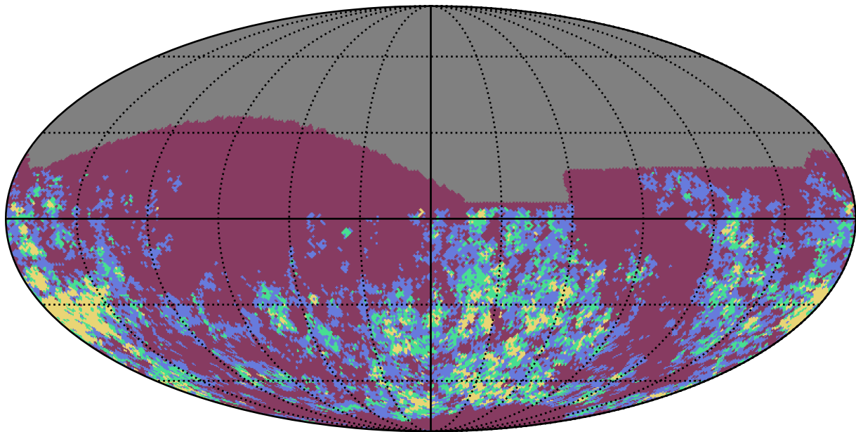
no_high_blob_v3.3_10yrs z band: Gaps_7hr
