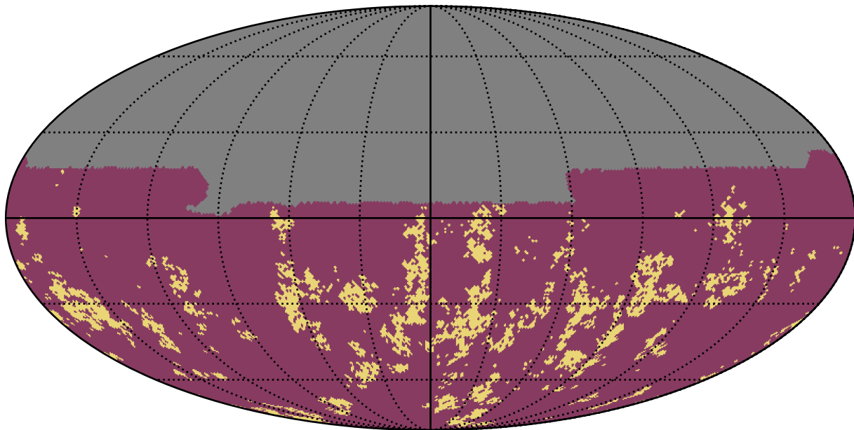
no_high_blob_v3.3_10yrs u band: Gaps_7hr
