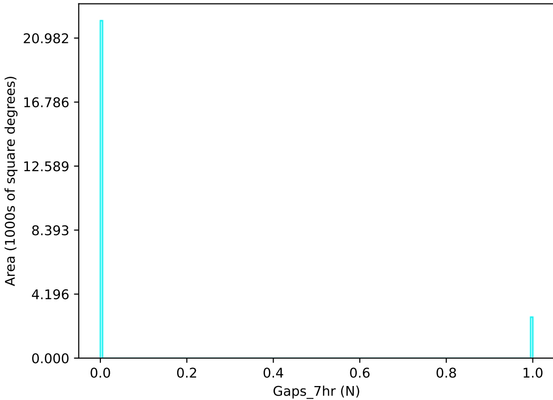
no_high_blob_v3.3_10yrs u band: Gaps_7hr
