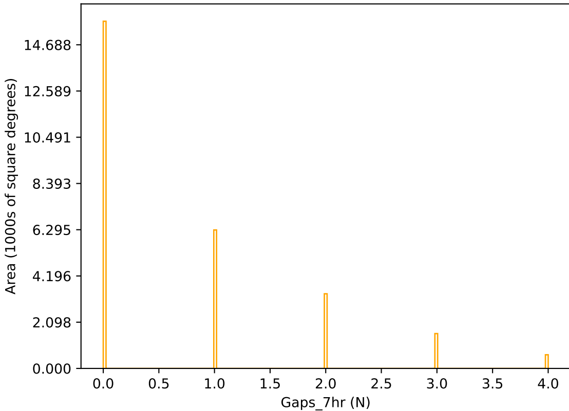
no_high_blob_v3.3_10yrs r band: Gaps_7hr
