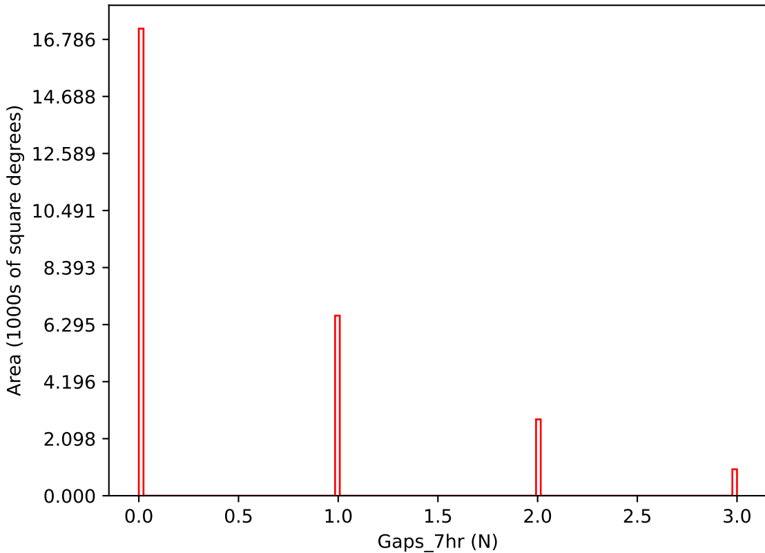
no_high_blob_v3.3_10yrs i band: Gaps_7hr
