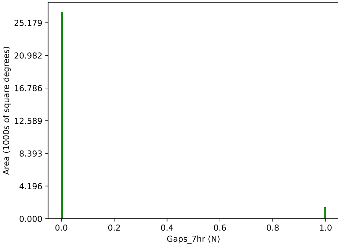
no_high_blob_v3.3_10yrs g band: Gaps_7hr
