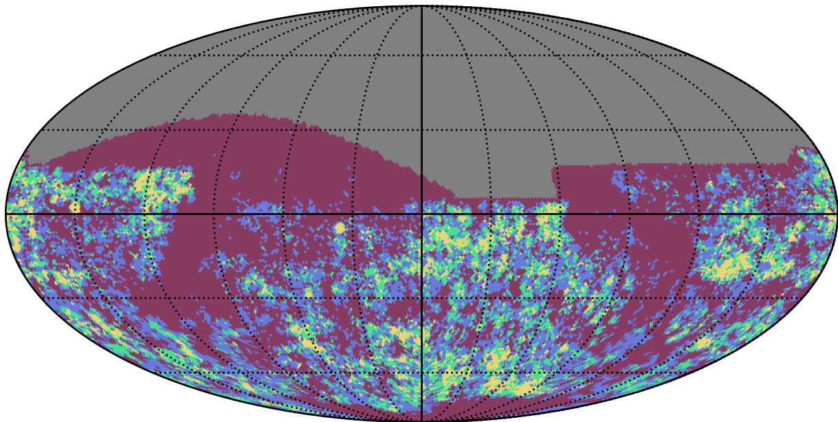
no_high_blob_v3.3_10yrs z band: Gaps_3hr
