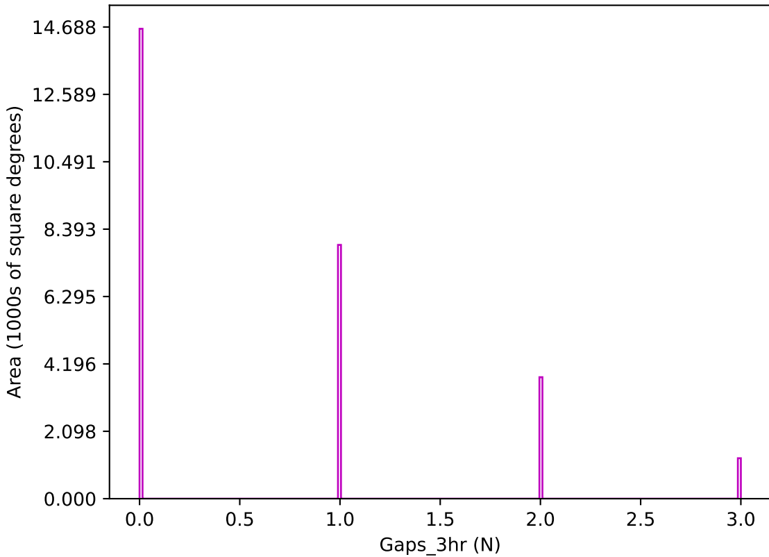
no_high_blob_v3.3_10yrs z band: Gaps_3hr
