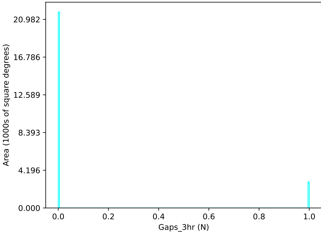
no_high_blob_v3.3_10yrs u band: Gaps_3hr
