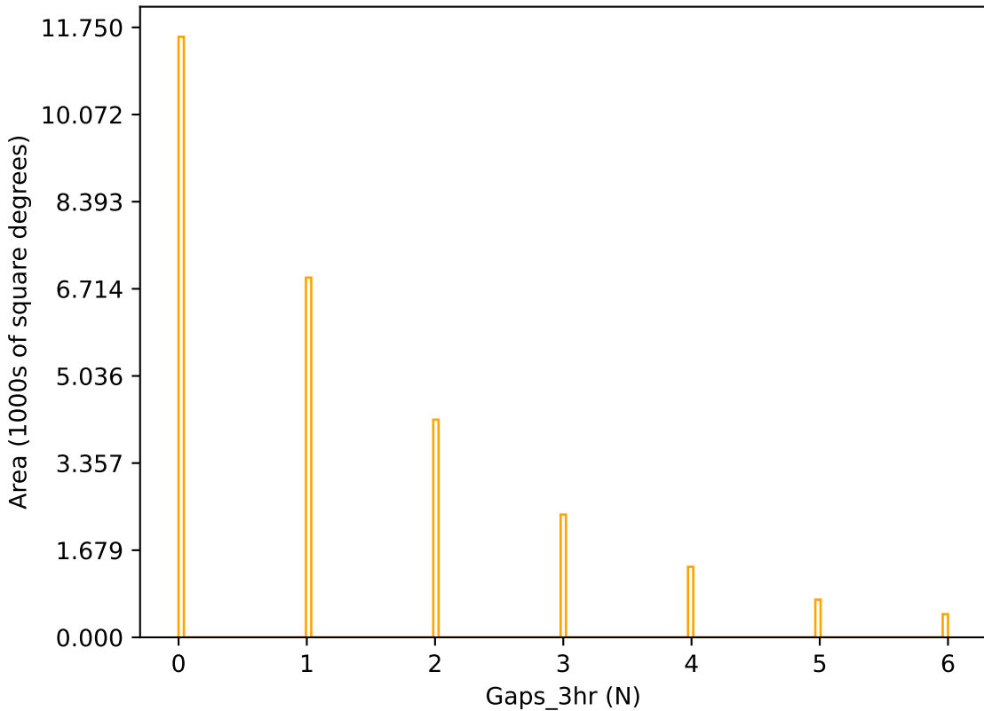
no_high_blob_v3.3_10yrs r band: Gaps_3hr
