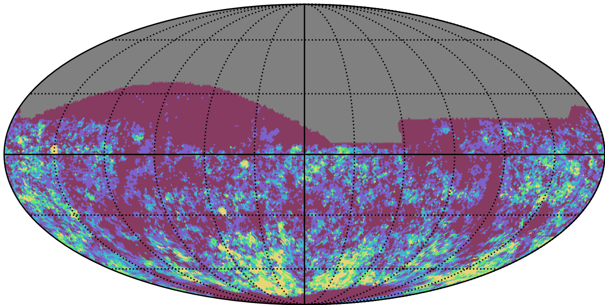
no_high_blob_v3.3_10yrs i band: Gaps_3hr
