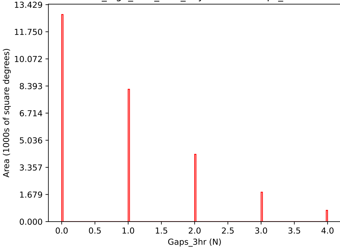
no_high_blob_v3.3_10yrs i band: Gaps_3hr
