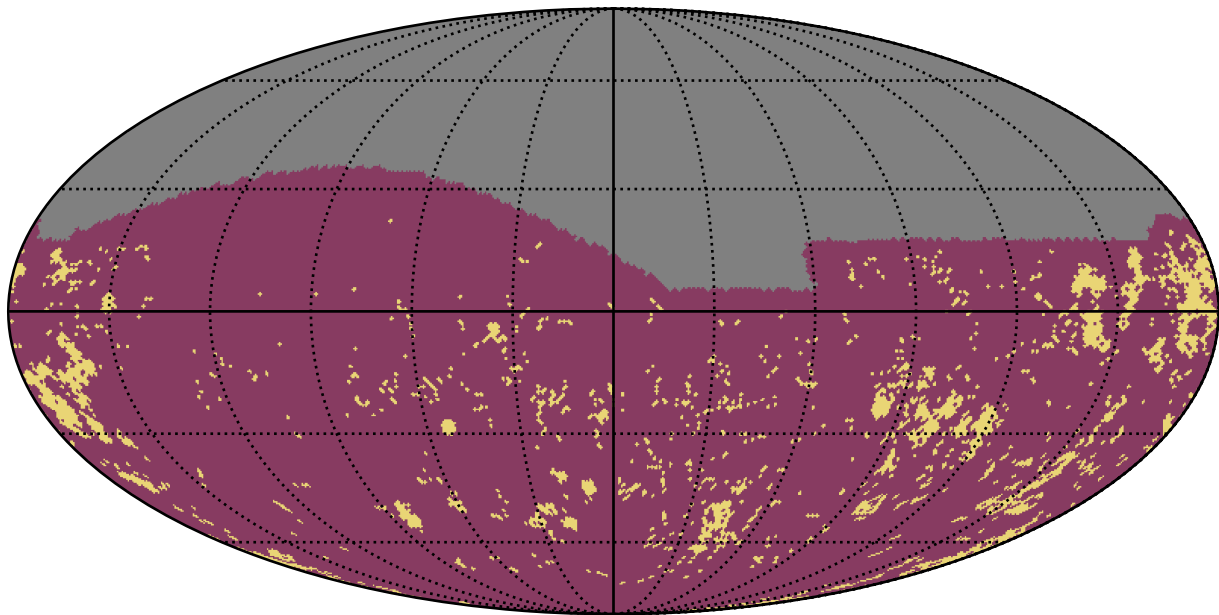
no_high_blob_v3.3_10yrs g band: Gaps_3hr
