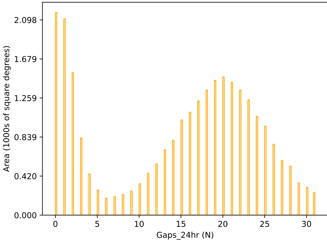
no_high_blob_v3.3_10yrs r band: Gaps_24hr
