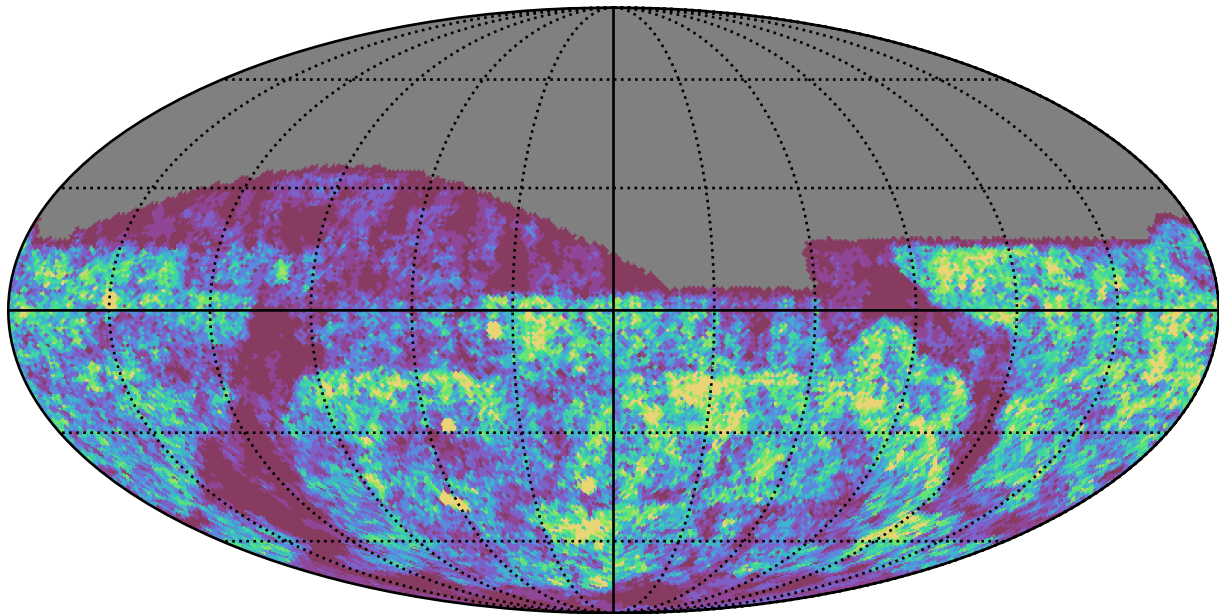
no_high_blob_v3.3_10yrs g band: Gaps_24hr
