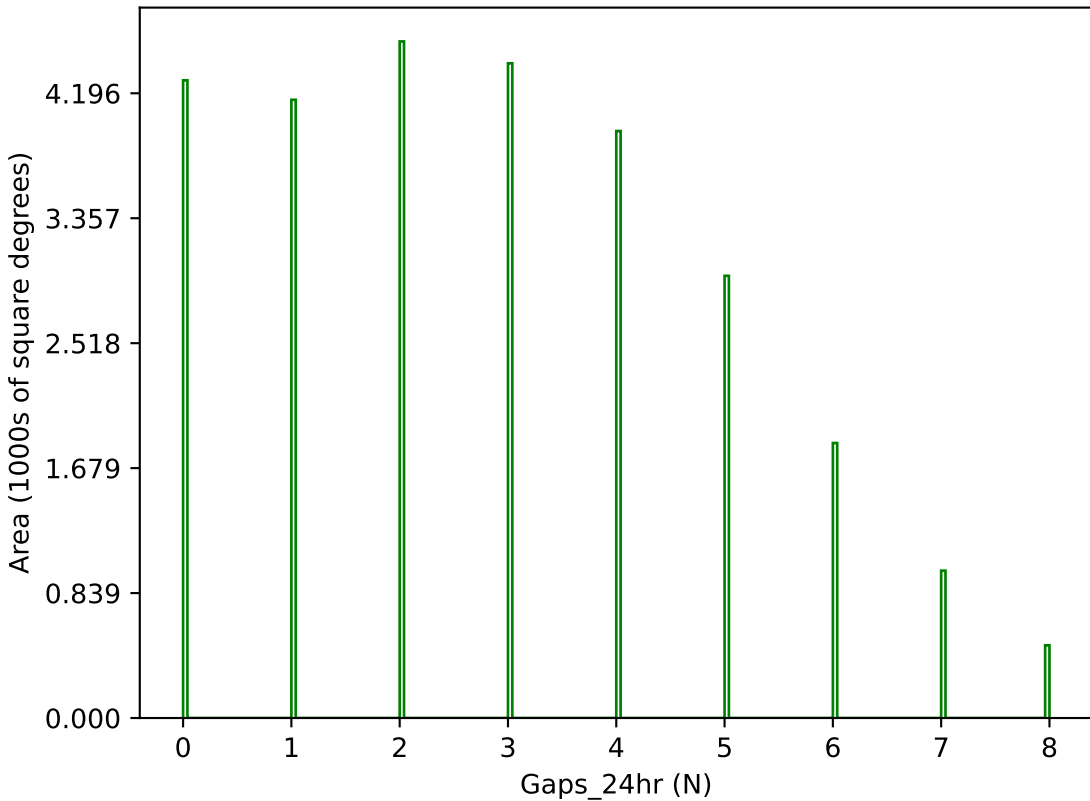
no_high_blob_v3.3_10yrs g band: Gaps_24hr
