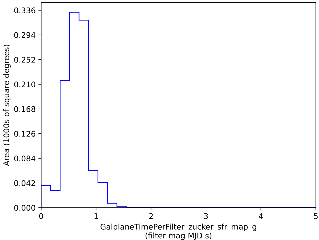
no_high_blob_v3.3_10yrs : GalplaneTimePerFilter_zucker_sfr_map_g
