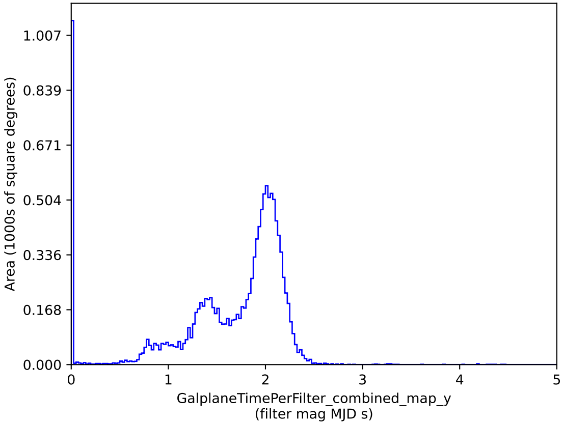
no_high_blob_v3.3_10yrs : GalplaneTimePerFilter_combined_map_y
