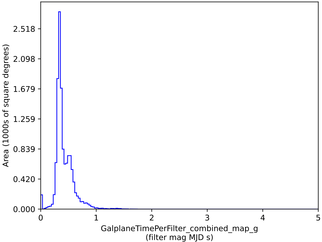
no_high_blob_v3.3_10yrs : GalplaneTimePerFilter_combined_map_g
