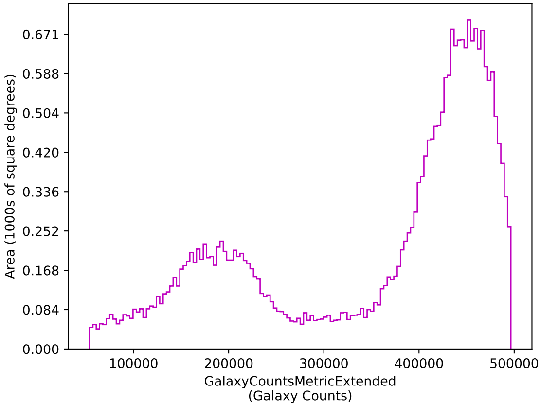
no_high_blob_v3.3_10yrs z: GalaxyCountsMetricExtended
