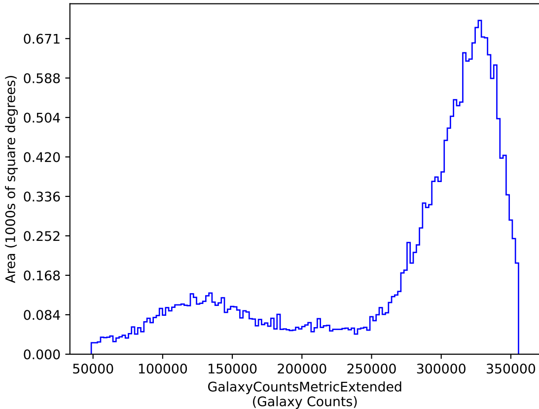
no_high_blob_v3.3_10yrs y: GalaxyCountsMetricExtended
