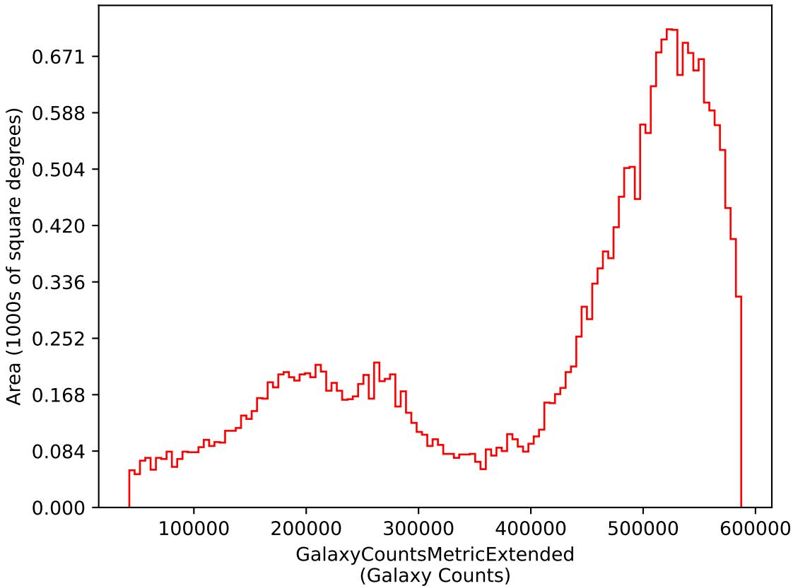
no_high_blob_v3.3_10yrs i: GalaxyCountsMetricExtended
