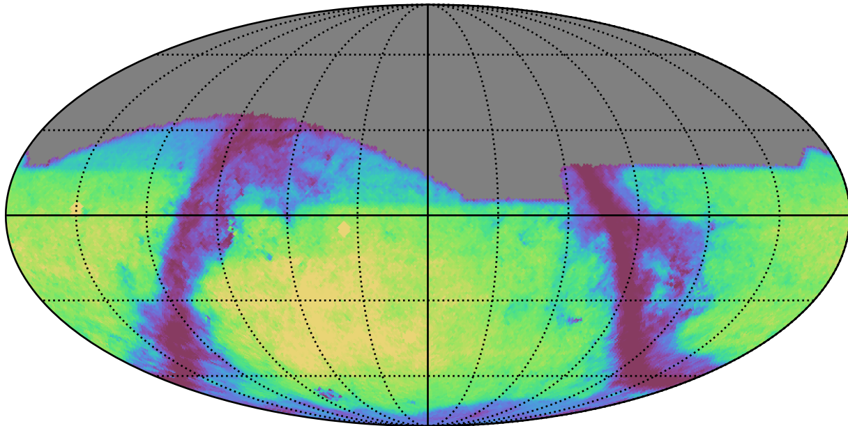
no_high_blob_v3.3_10yrs g: GalaxyCountsMetricExtended
