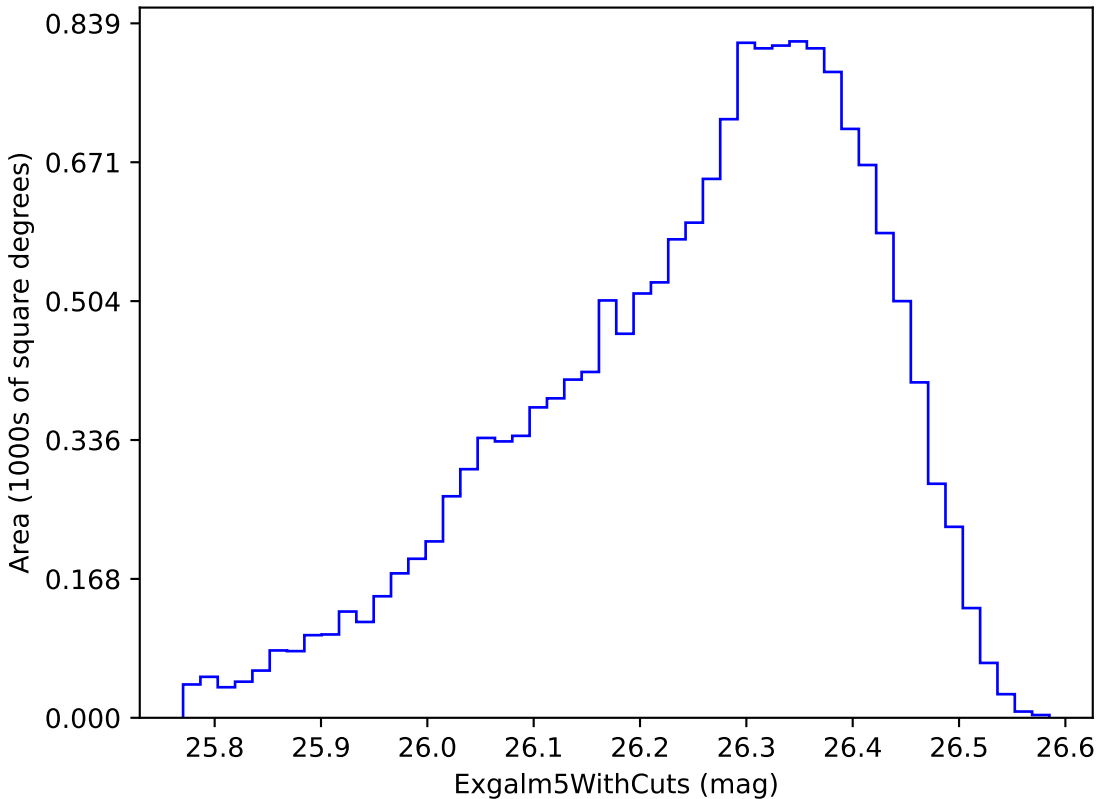
no_high_blob_v3.3_10yrs i band non-DD year 8: Exgalml5WithCuts
