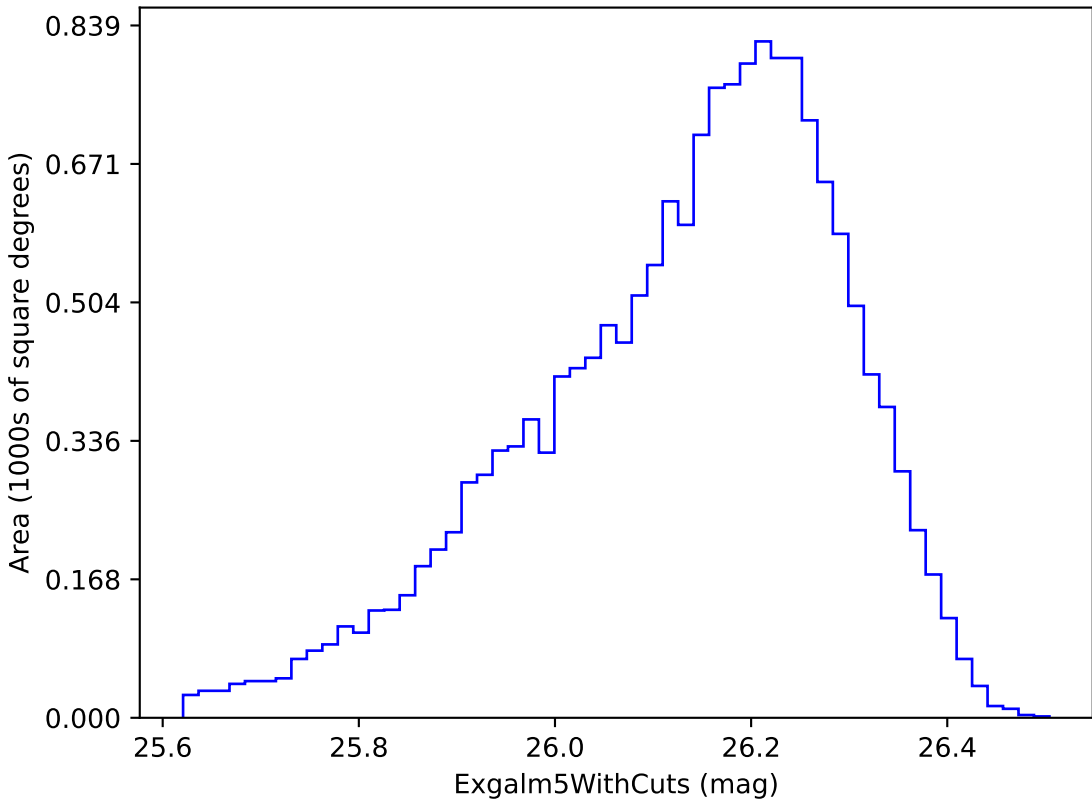
no_high_blob_v3.3_10yrs i band non-DD year 6: Exgalml5WithCuts
