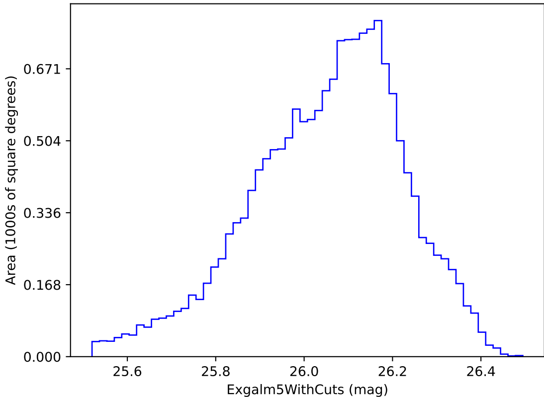
no_high_blob_v3.3_10yrs i band non-DD year 5: Exgalml5WithCuts
