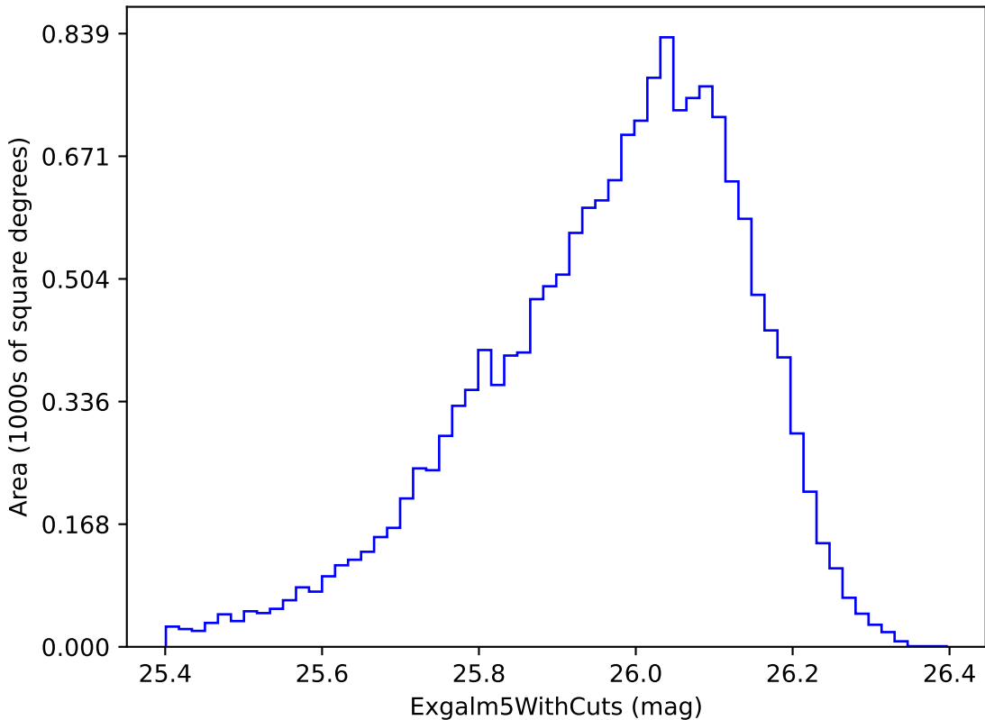
no_high_blob_v3.3_10yrs i band non-DD year 4: Exgalml5WithCuts
