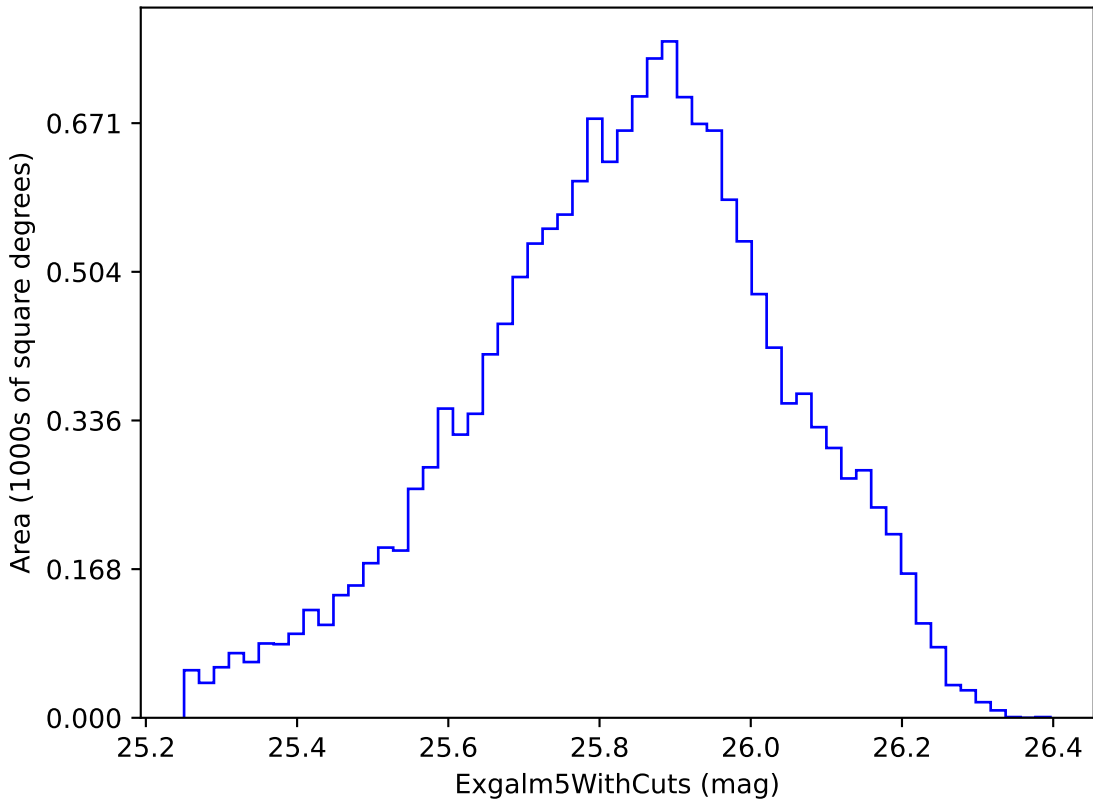
no_high_blob_v3.3_10yrs i band non-DD year 3: Exgalml5WithCuts
