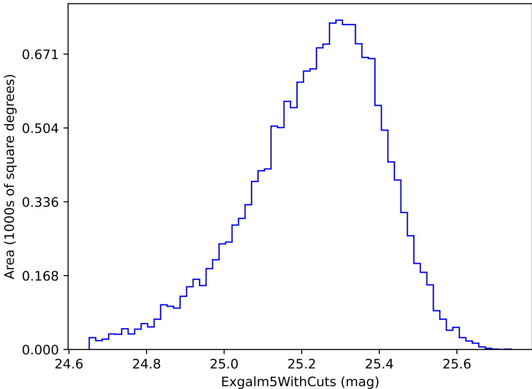
no_high_blob_v3.3_10yrs i band non-DD year 1: Exgalml5WithCuts
