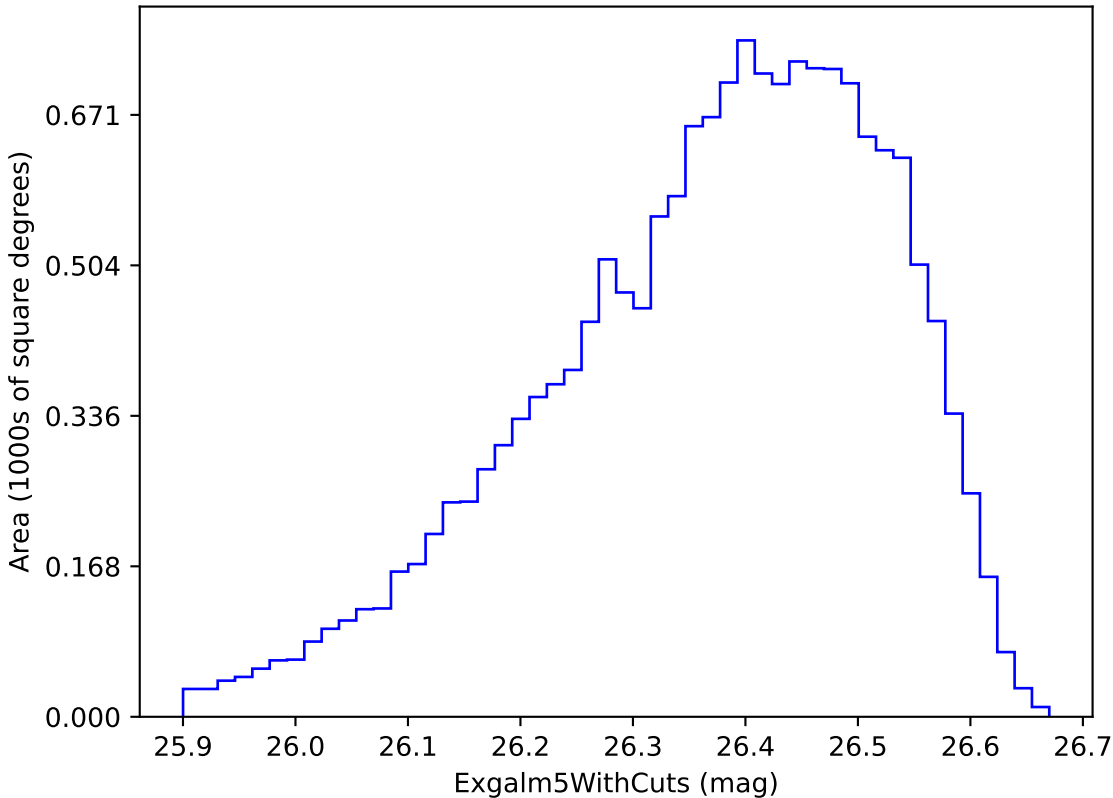
no_high_blob_v3.3_10yrs i band non-DD year 10: ExgalM5WithCuts
