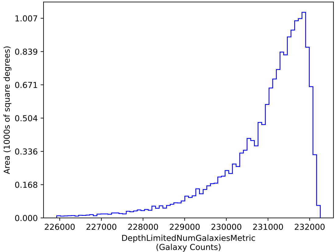
no_high_blob_v3.3_10yrs i band galaxies non-DD: DepthLimitedNumGalaxiesMetric
