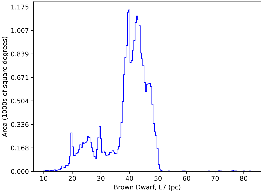
no_high_blob_v3.3_10yrs : Brown Dwarf, L7
