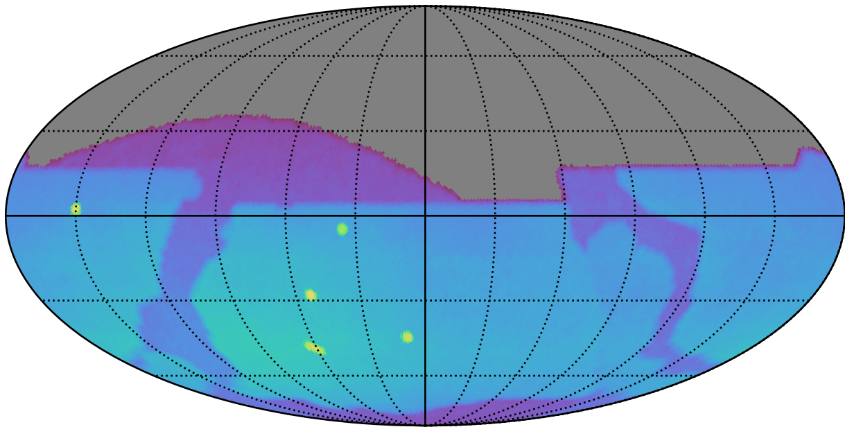
no_high_blob_v3.3_10yrs : Brown Dwarf, L4
