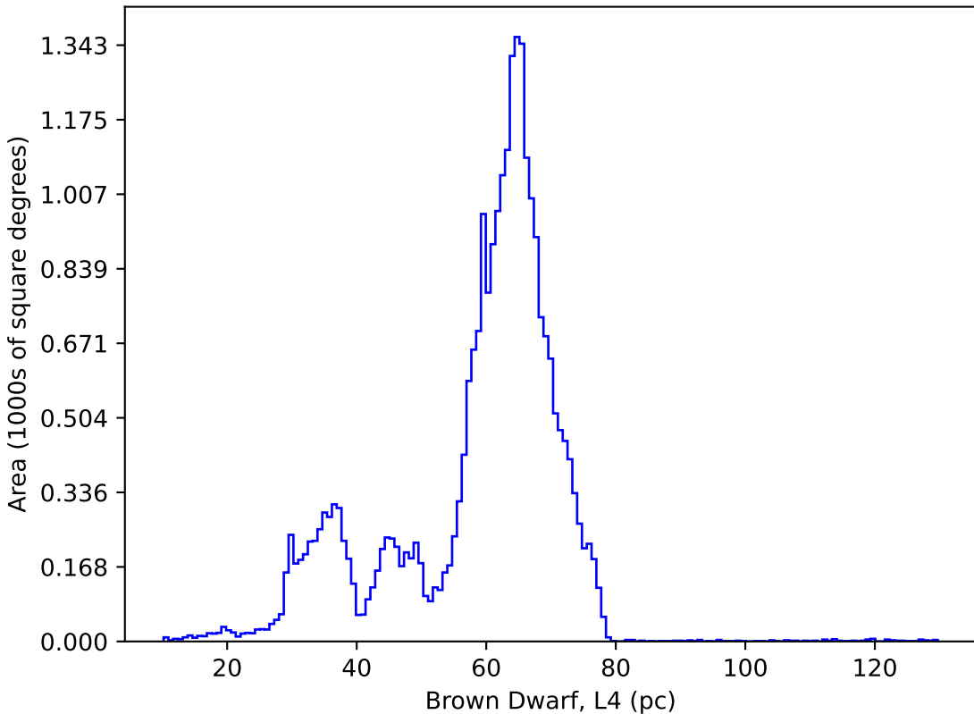
no_high_blob_v3.3_10yrs : Brown Dwarf, L4
