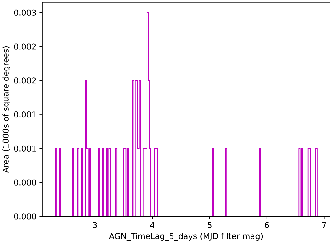
no_high_blob_v3.3_10yrs z band: AGN_TimeLag_5_days
