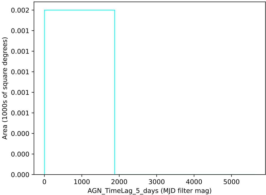
no_high_blob_v3.3_10yrs u band: AGN_TimeLag_5_days
