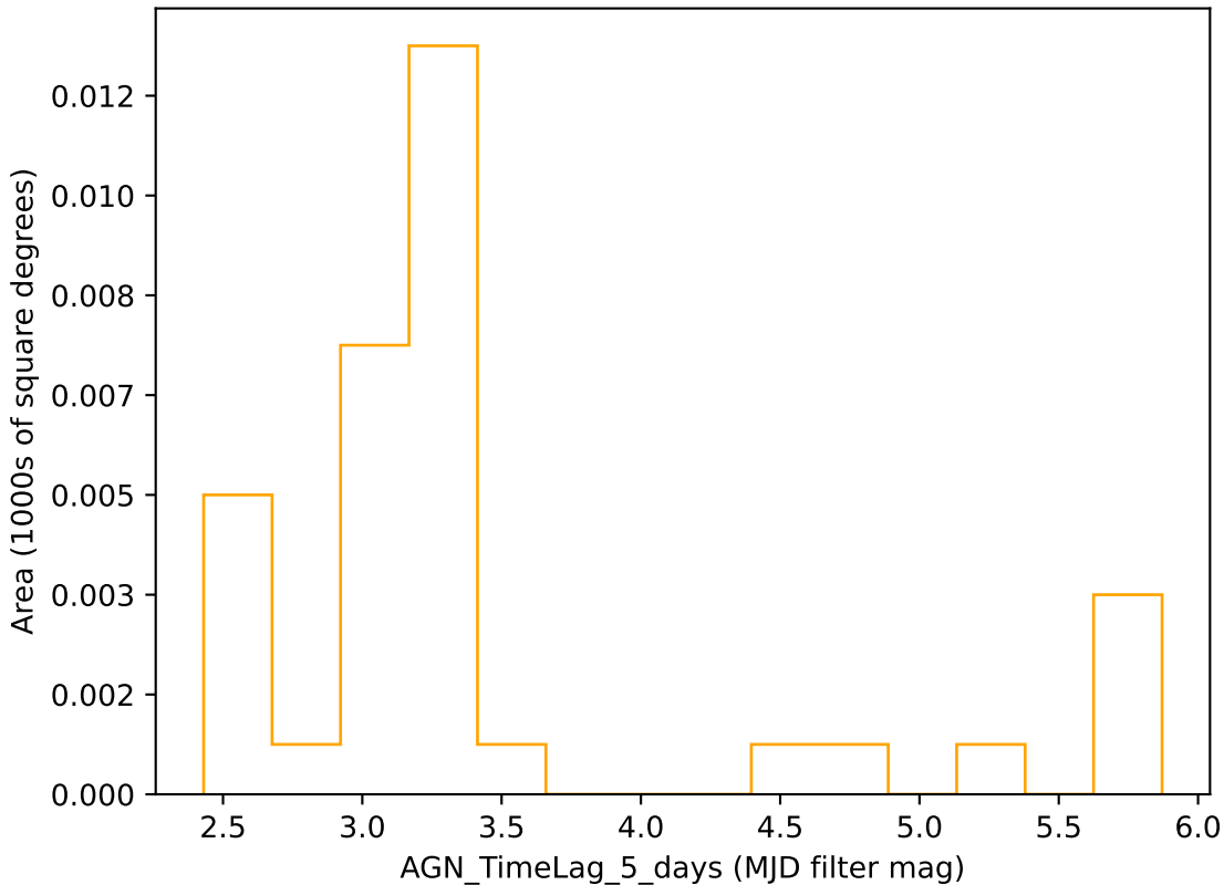
no_high_blob_v3.3_10yrs r band: AGN_TimeLag_5_days
